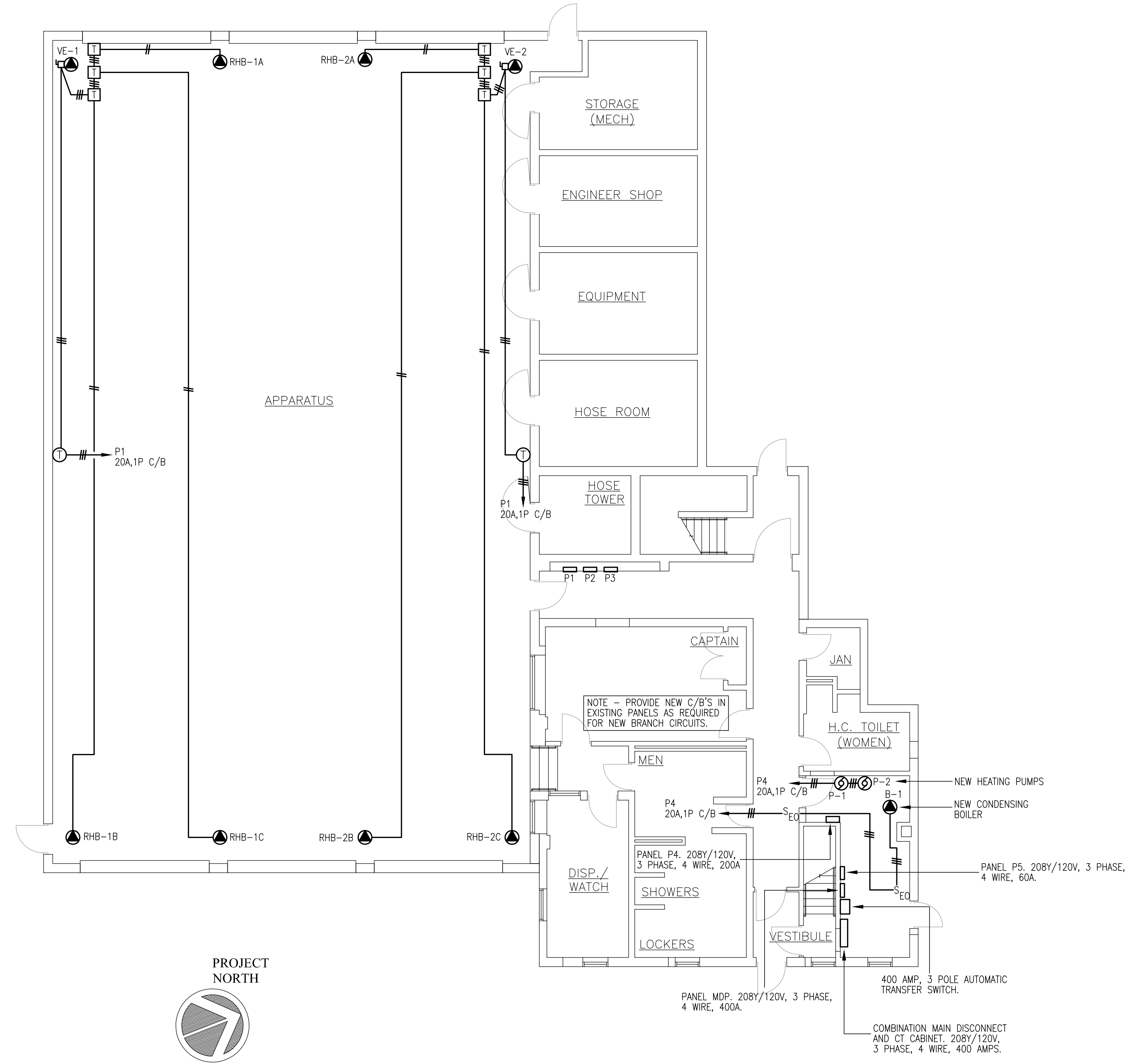
FIRE HOUSE #2 FLOOR PLAN - NEW WORK SCALE: 1/8"=1'-0"
