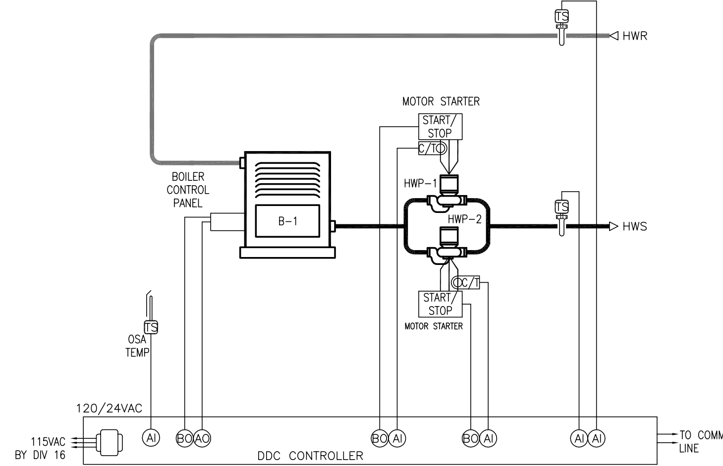
BOILER CONTROLS DIAGRAM NO SCALE
