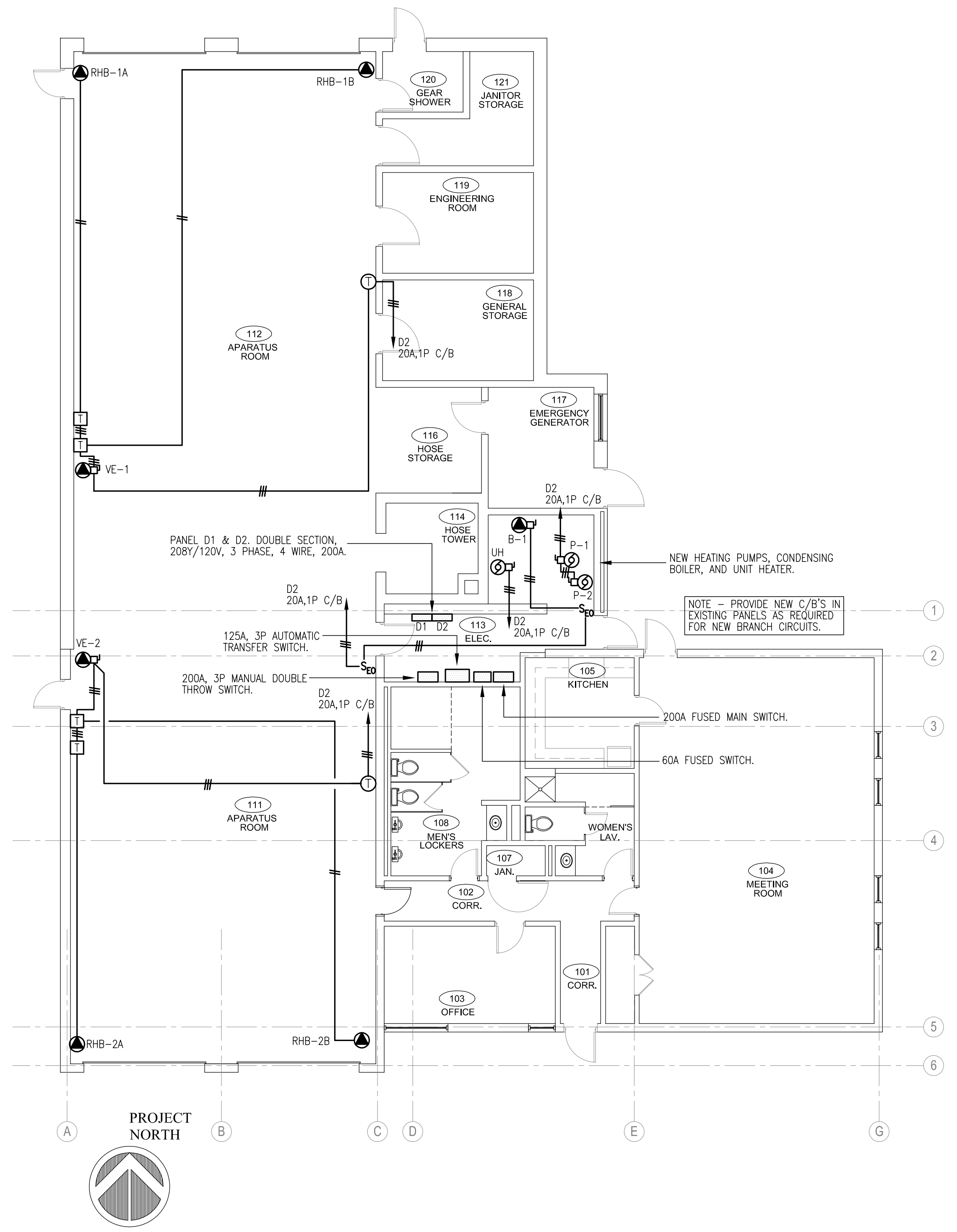
FIRE HOUSE #3 FLOOR PLAN - NEW WORK SCALE: 1/8" = 1'-0"
