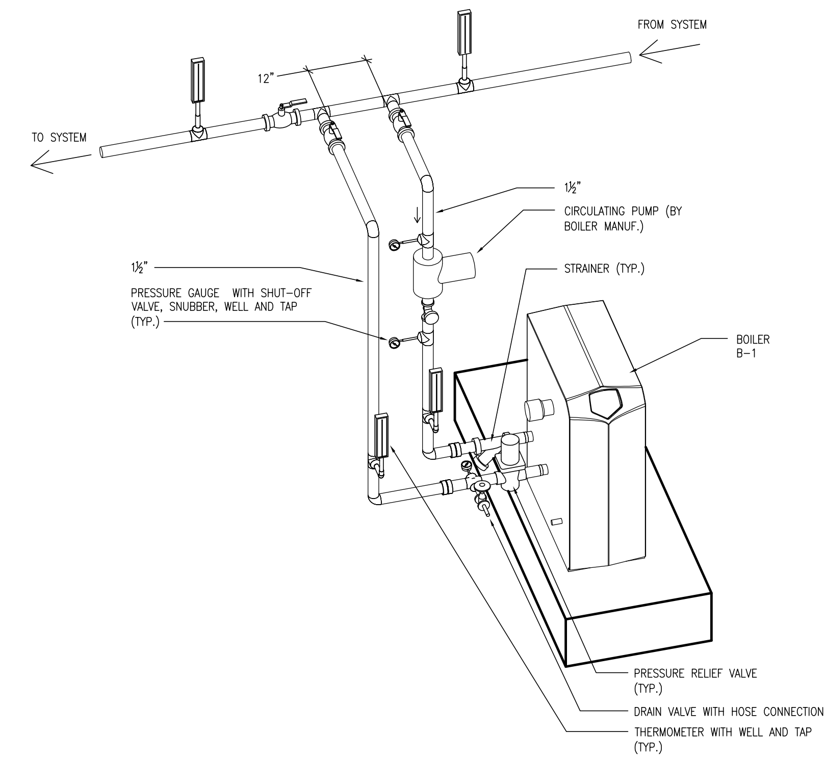
BOILER PIPING DETAIL NO SCALE
