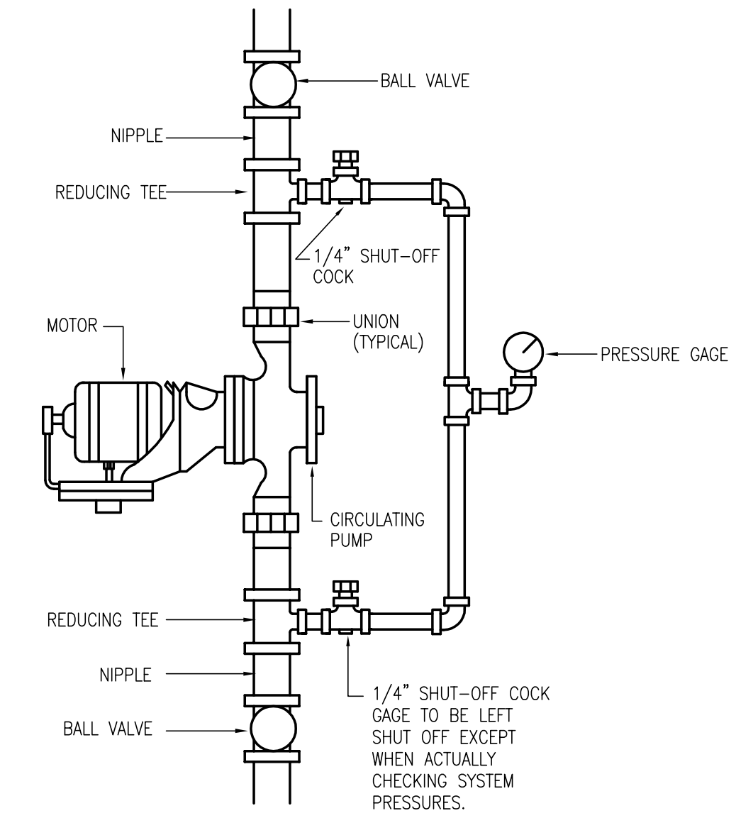
INSTALLATION DETAILS OF IN-LINE CIRCULATING PUMP NO SCALE
