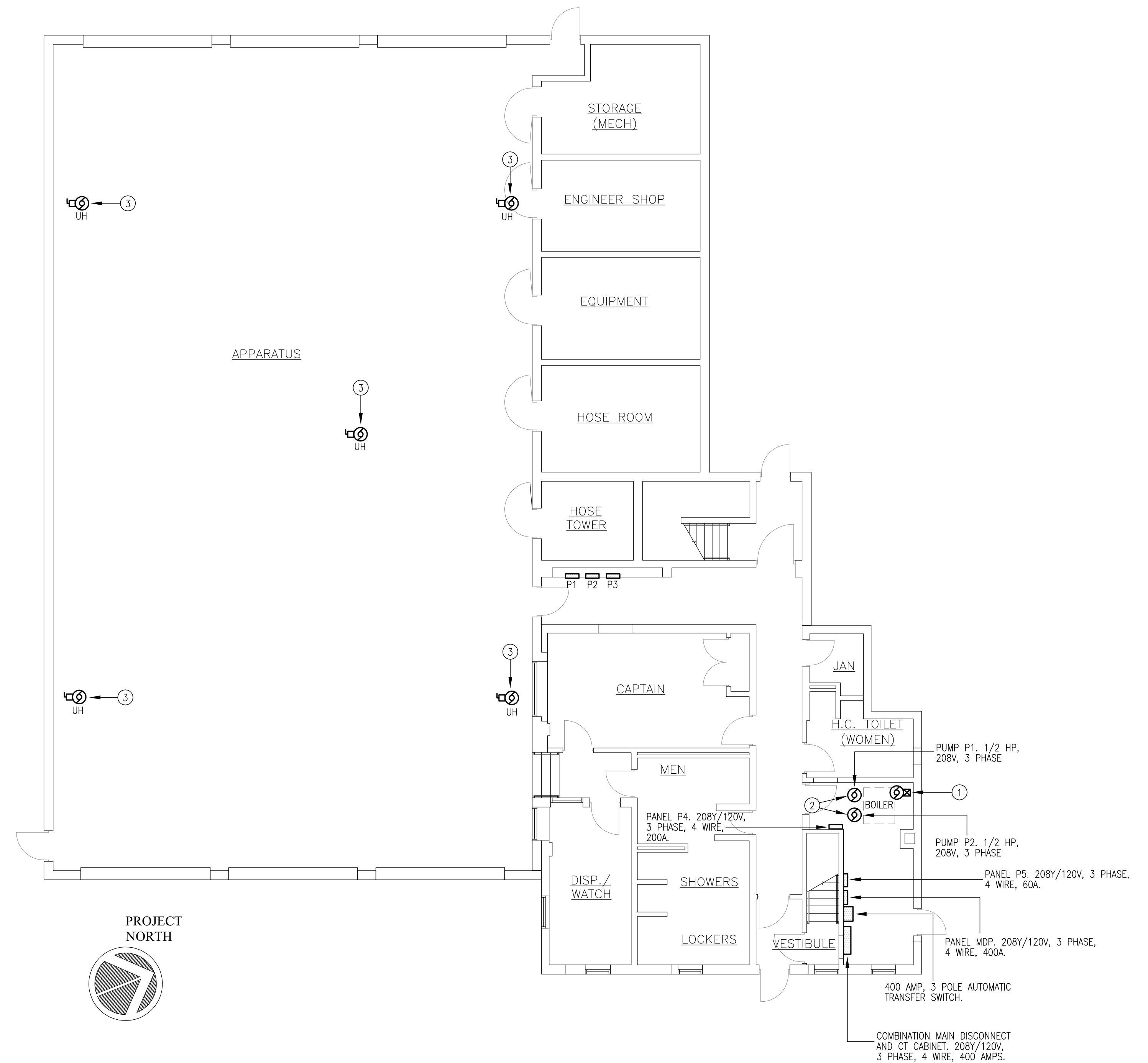
FIRE HOUSE #2 FLOOR PLAN - DEMOLITION SCALE: 1/8"=1'-0"
