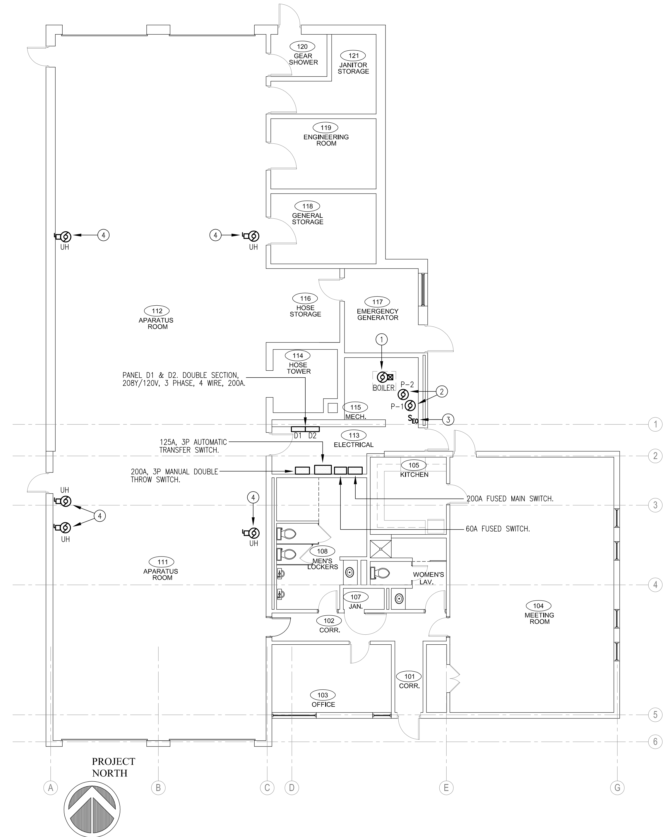
FIRE HOUSE #3 FLOOR PLAN - DEMOLITION SCALE: 1/8"=1'-0"
