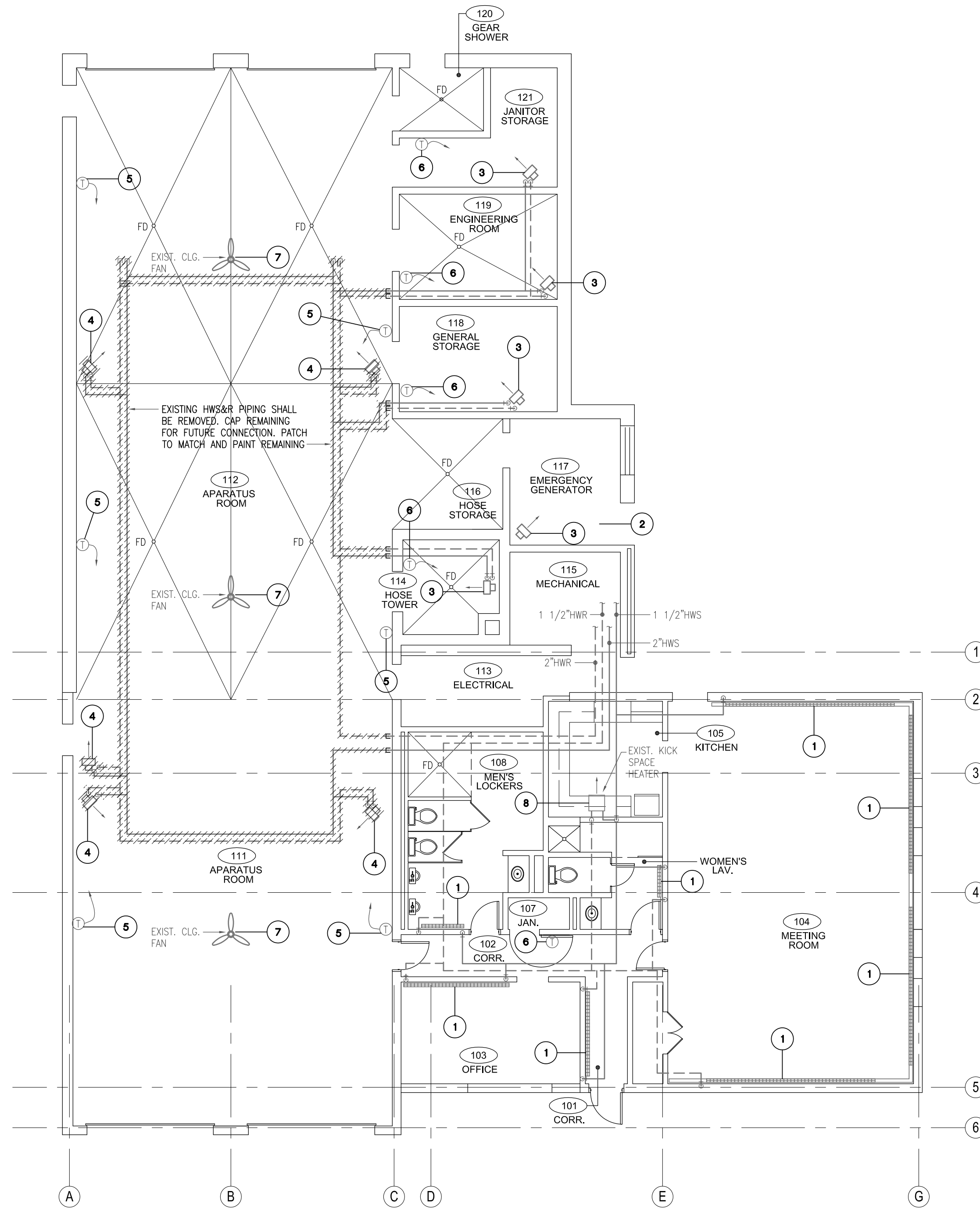
FLOOR PLAN - MECHANICAL DEMOLITION SCALE: 1/8"=1'-0"
