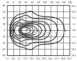
OSQ-HO-A**-25D-40L-40K-UL Mounting Height: 25' (7.6m) A.F.G., 60° Tilt Initial Delivered Lumens: 41,542 Initial FC at grade
