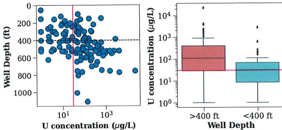
Figure 5. Uranium concentration and well depth. On the left, a scatterplot shows the plotted data from Glastonbury with a red line for a uranium concentration of 30 ug/L and a dotted black line indicating the median well depth from the Glastonbury data (~400 ft). On the right, two boxplots show the distribution of measured uranium concentrations in wells less than 400 ft deep and well greater than 400 ft deep.
