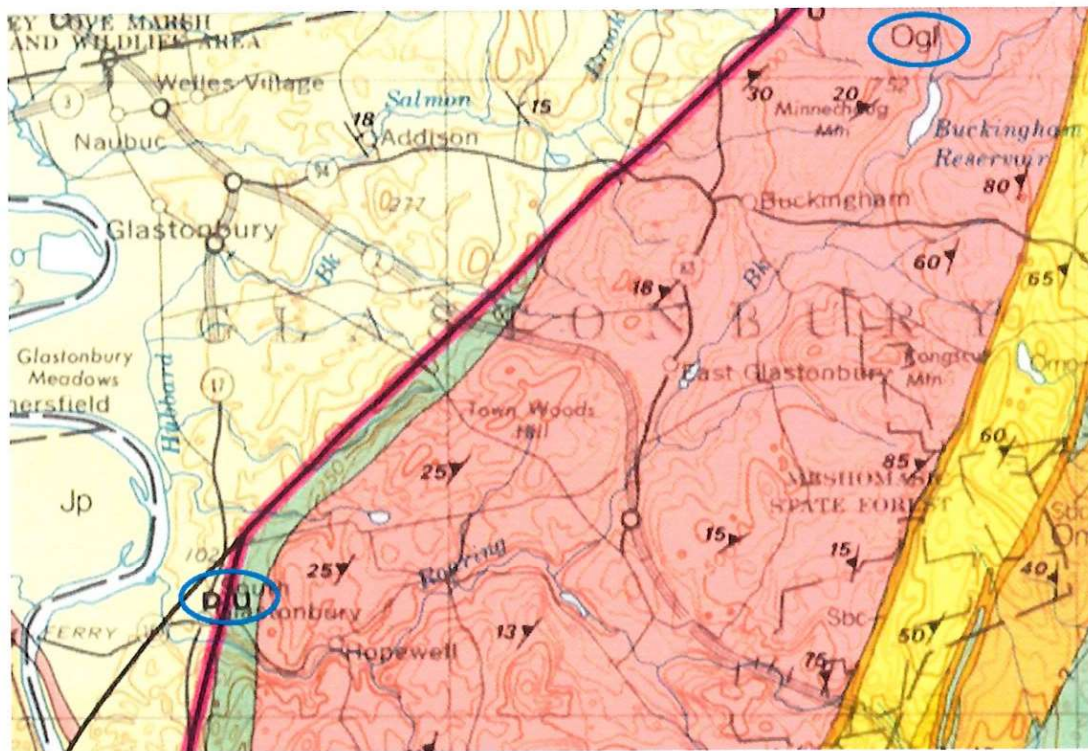
Figure 1: Bedrock geologic map of Connecticut showing Glastonbury portion. “Ogl” is the Glastonbury Gneiss unit, “U” is the upthrown block of high-angle fault, and “D” is the downthrown block of high-angle fault.
