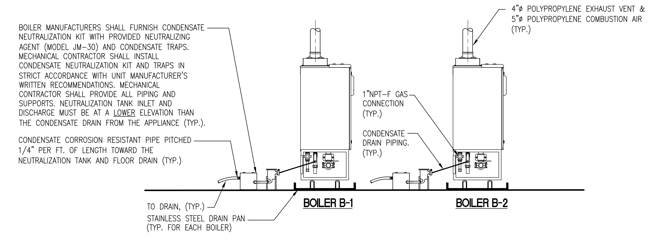
TYPICAL GAS FIRED BOILER VENTING AND CONDENSATE DETAIL NO SCALE
