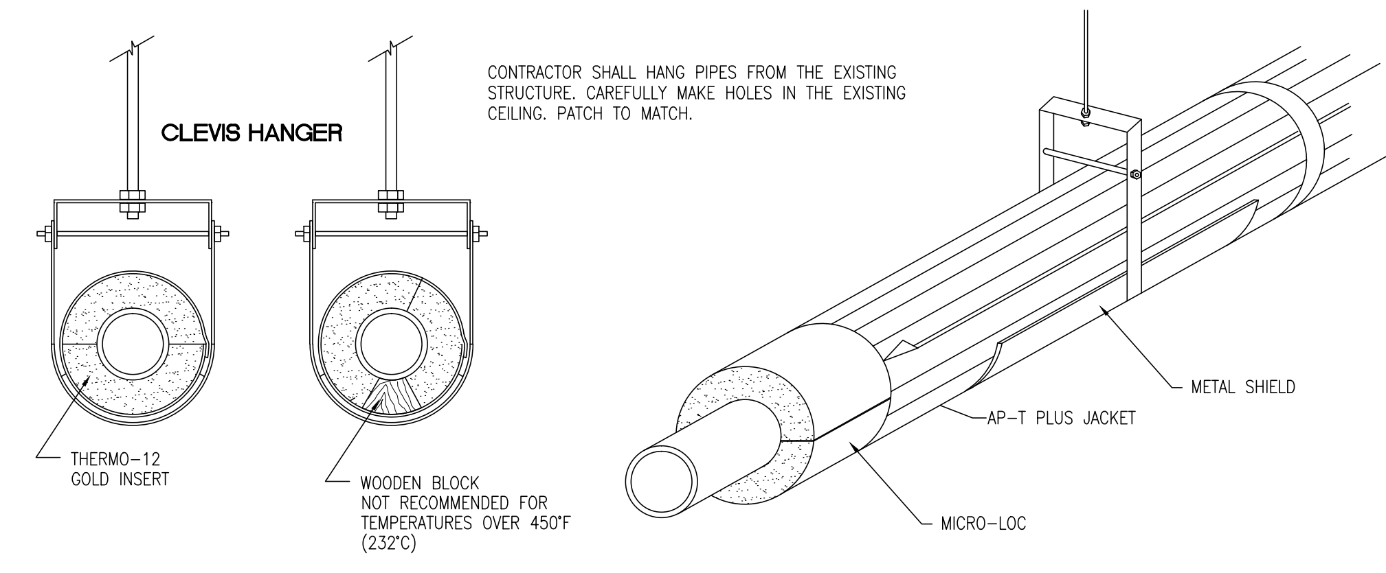
TYPICAL HOT WATER PIPING INSULATION NO SCALE
