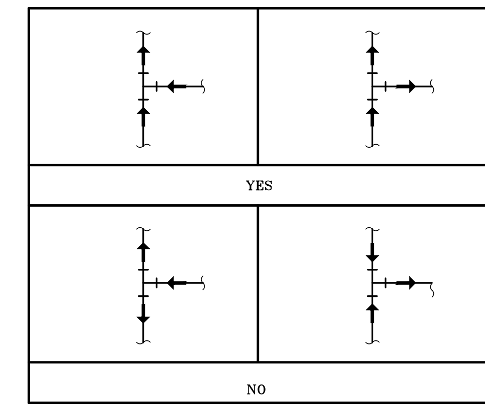
ALLOWABLE FLOW CONFIGURATIONS IN PIPING TEES-HVAC SYSTEMS NO SCALE
