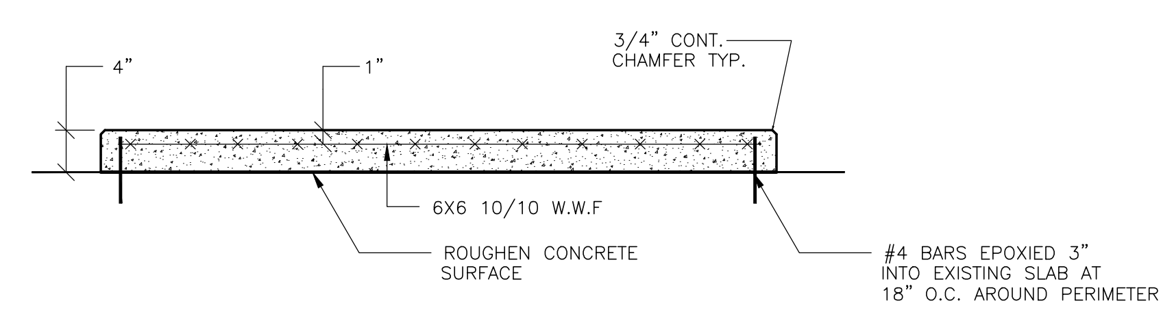
TYPICAL EQUIPMENT HOUSEKEEPING PAD DETAIL NOT TO SCALE (COORDINATE NUMBER AND LOCATIONS WITH MEP DRAWINGS) NOTE: COORDINATE PAD THICKNESS AT BOILERS w/ M.E.P.
