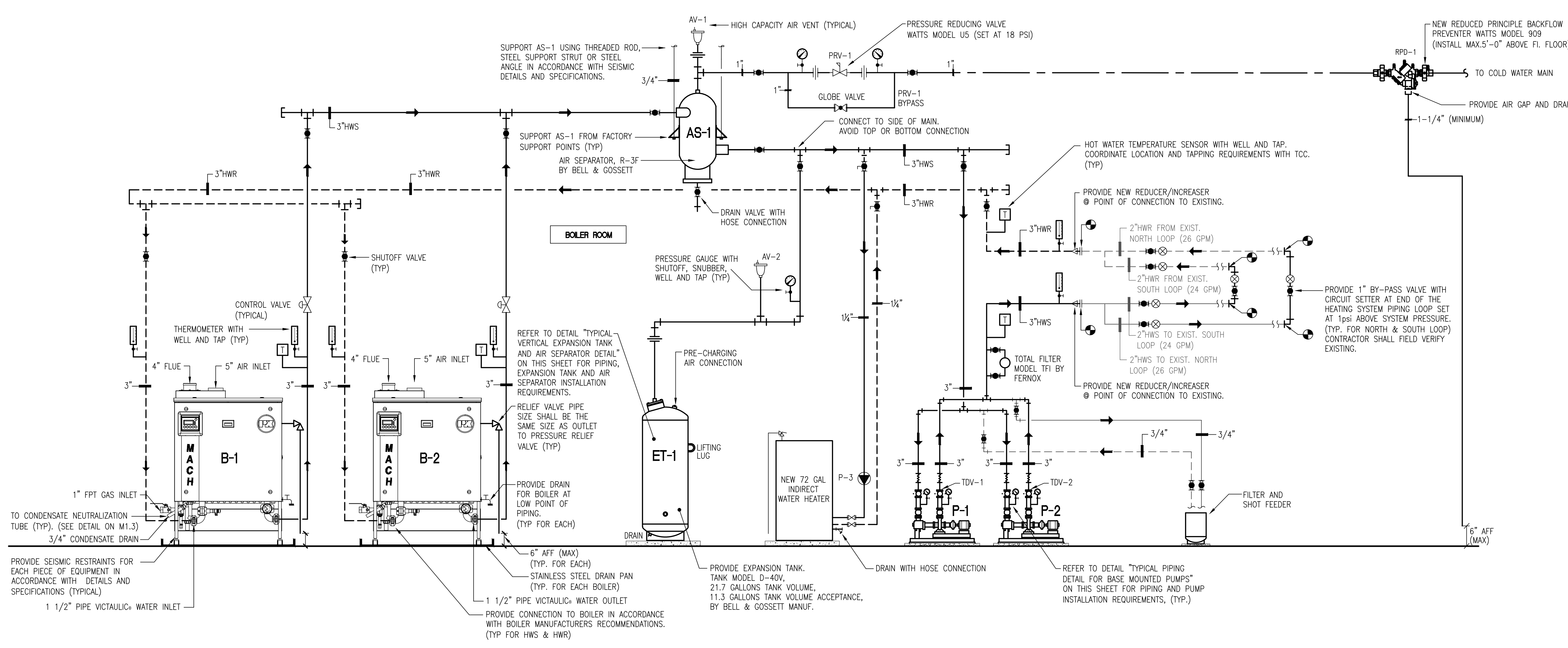
BOILER ROOM NEW HOT WATER PIPING DIAGRAM NO SCALE
