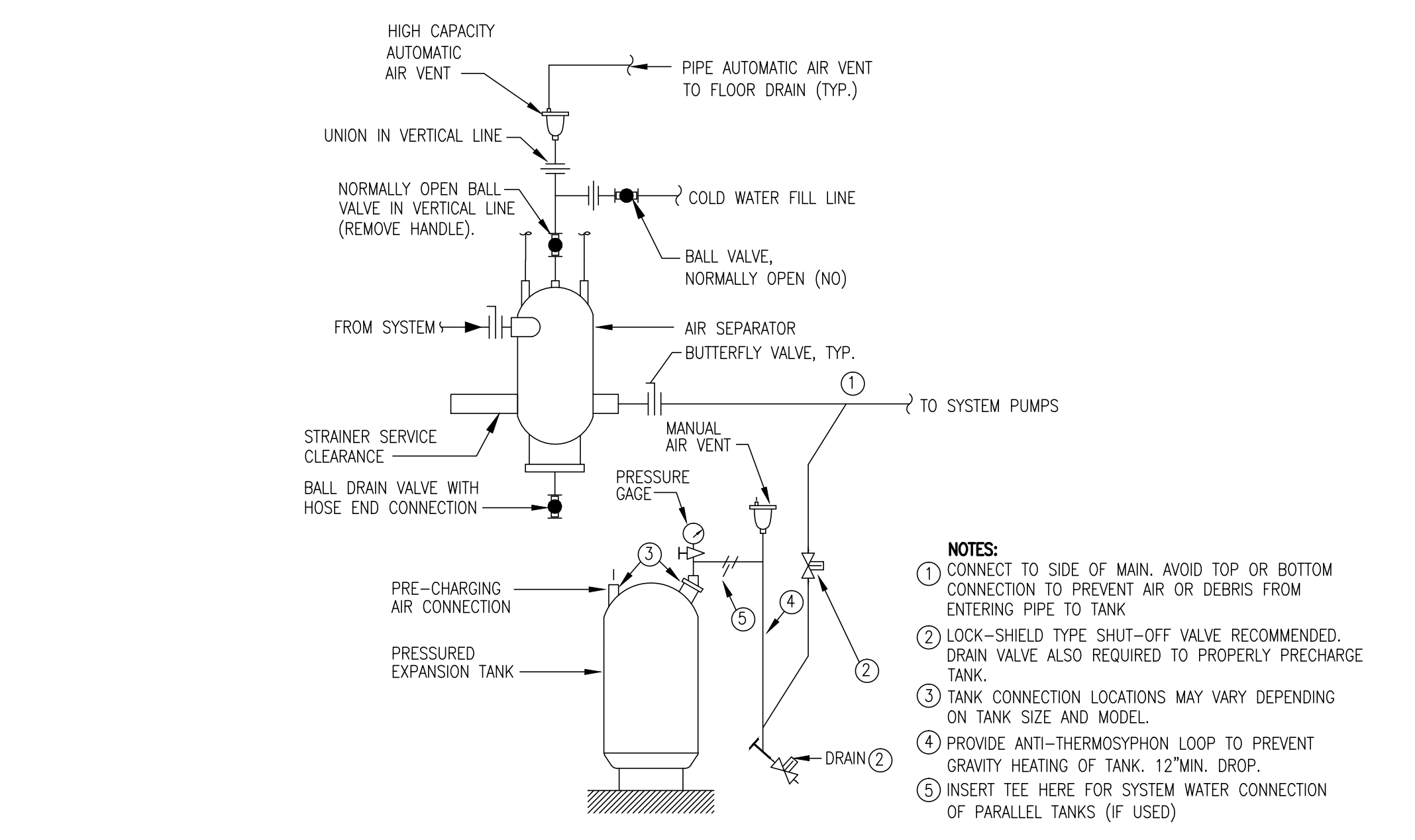
TYPICAL VERTICAL EXPANSION TANK WITH AIR SEPARATOR DETAIL NO SCALE
