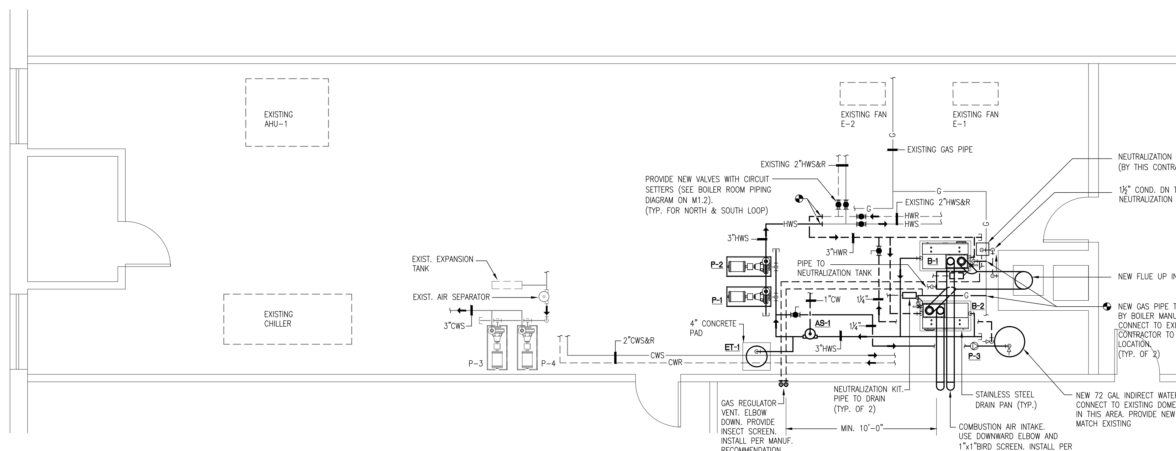
BOILER ROOM PART PLAN – MECHANICAL NEW WORK SCALE: 1/4"=1'-0"
