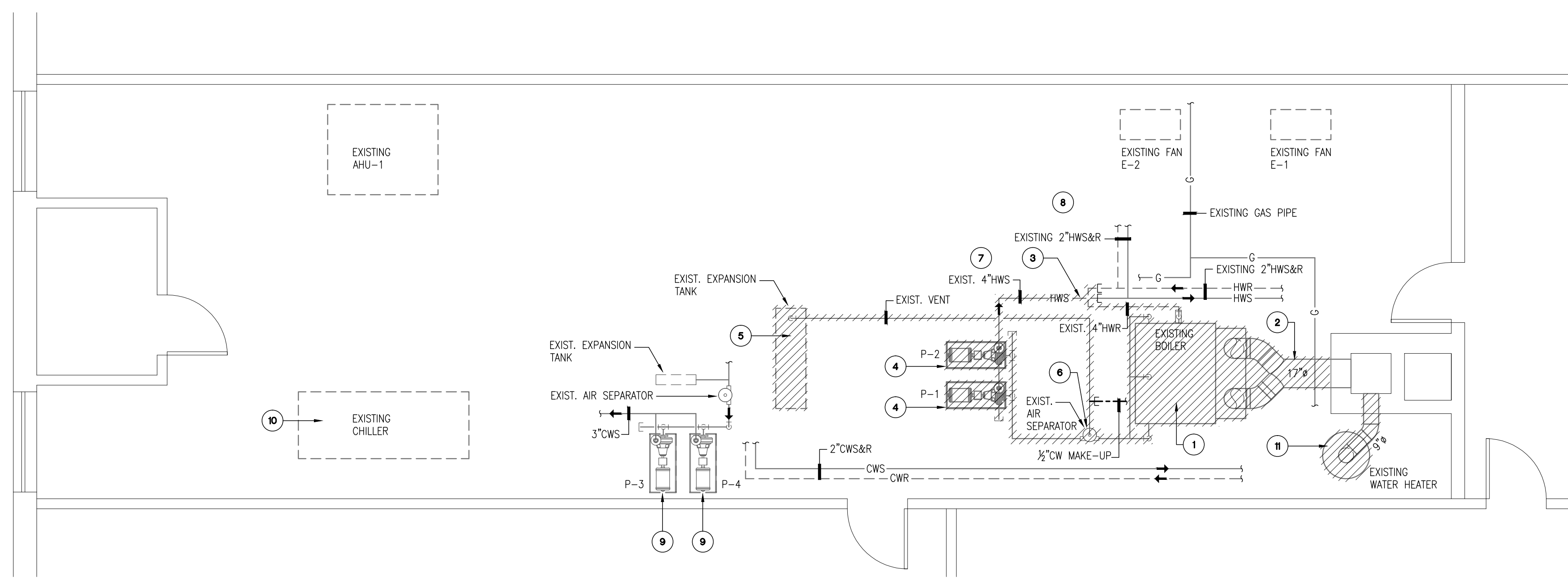
BOILER ROOM PART PLAN – MECHANICAL DEMOLITION SCALE: 1/4"=1'-0"
